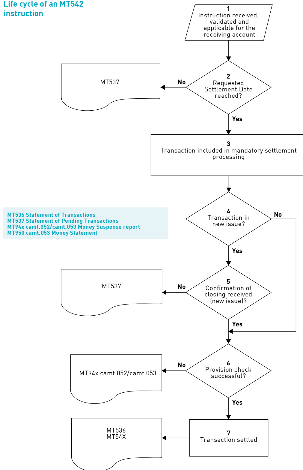
Figure 4.2 Life cycle of an MT542 instruction
