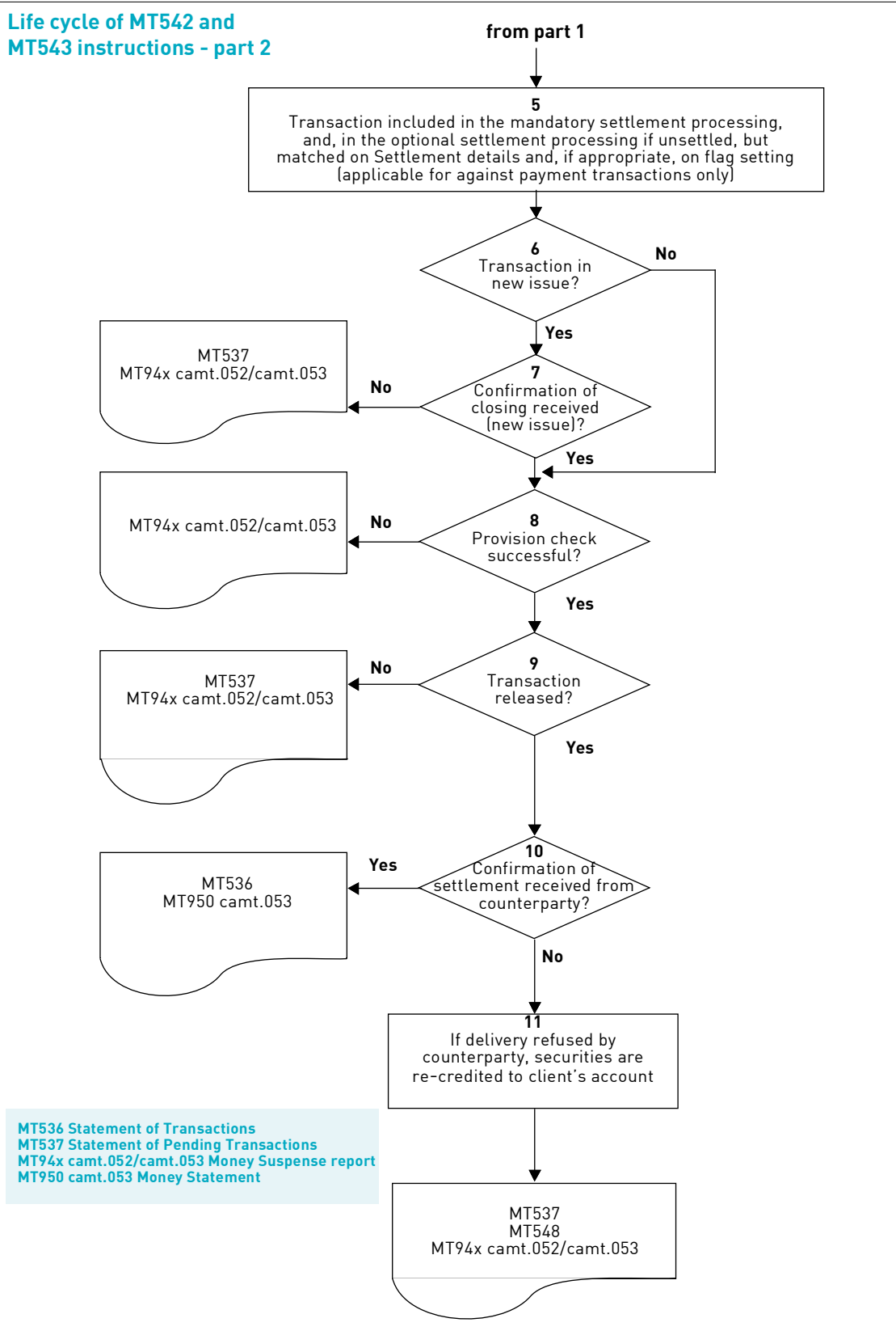
Figure 4.5 Life cycle of MT542 and MT543 instructions (Bridge deliveries) - part 2
