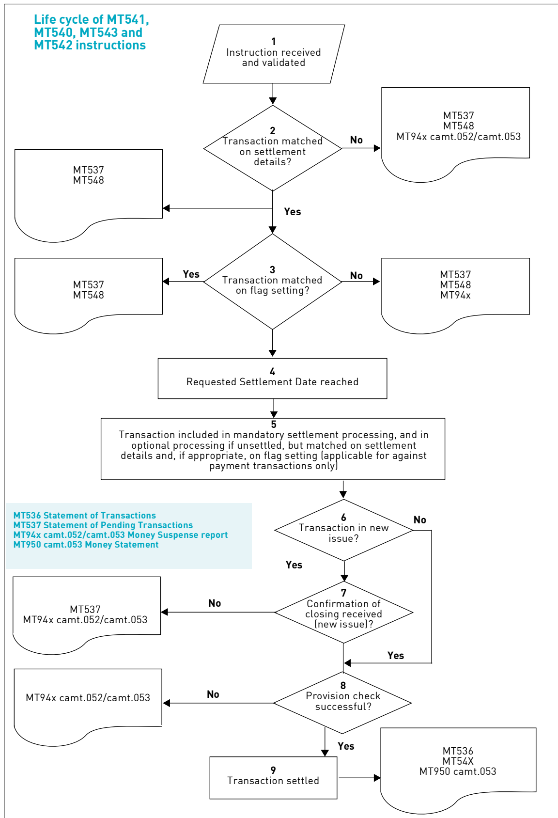
Figure 4.3 Life cycle of MT540, MT541, MT542 and MT543 instructions
